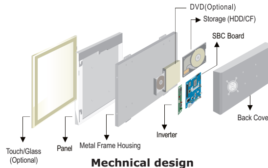
Mechanical design
